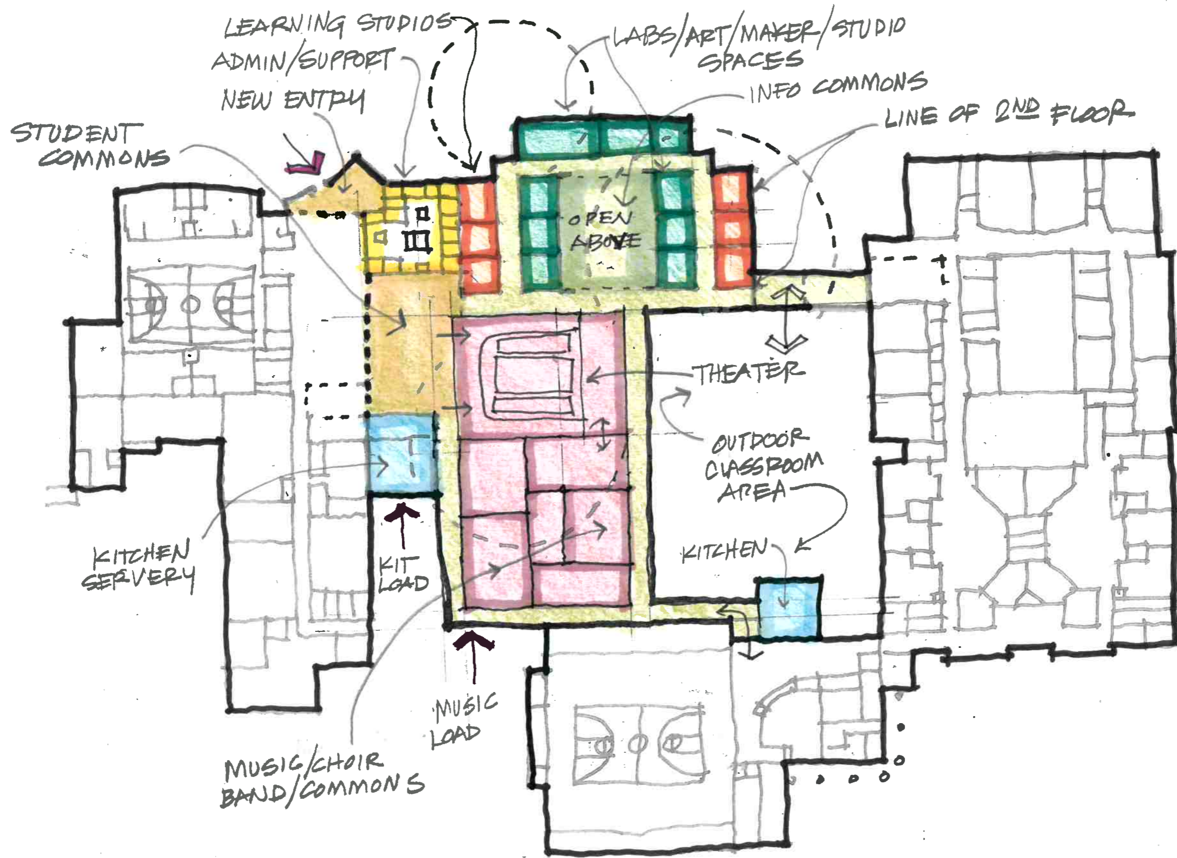
CHARLES CITY HIGH SCHOOL - FIRST FLOOR PLAN
